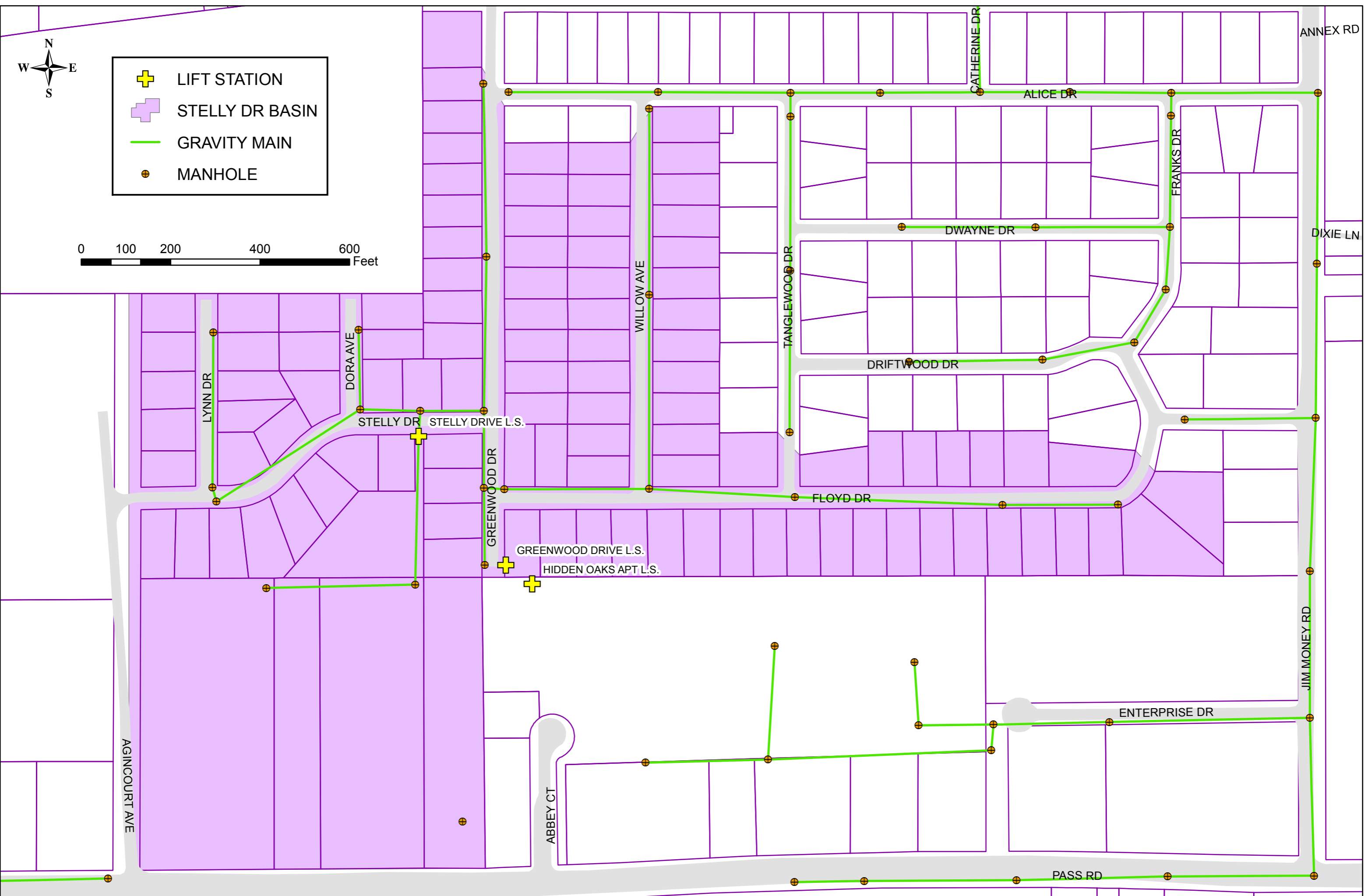
Stelly Lift Station Sewer Basin
